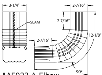
AAE923 A-Elbow
