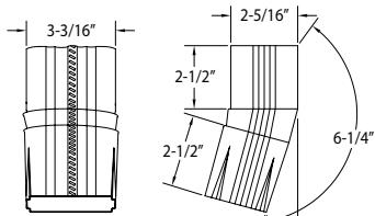
AAE123 A-Elbow
