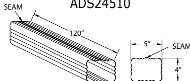
ADS24510
