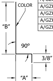
Z Flashing
